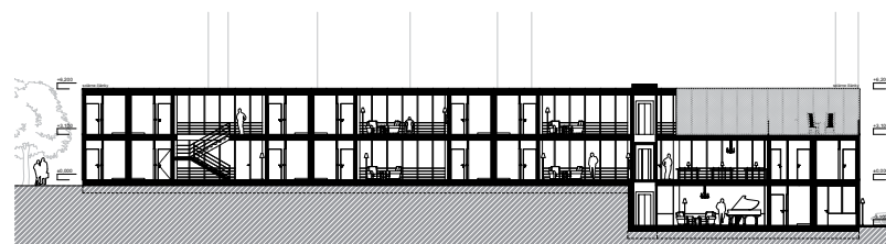
rez AA 1:200
